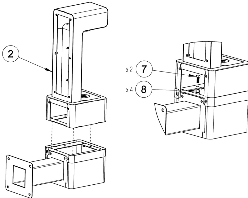
Fig.6 – Alcove assembly
