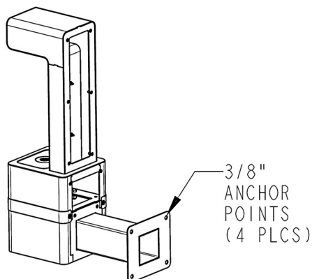
Fig.7 – Anchor points
